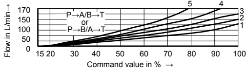
85L/min nominal flow at a 10 bar valve pressure differential
