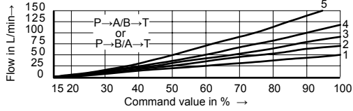
85L/min nominal flow at a 10 bar valve pressure differential
