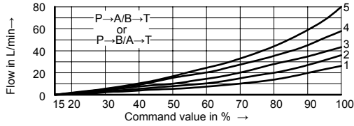
50L/min nominal flow at a 10 bar valve pressure differential
