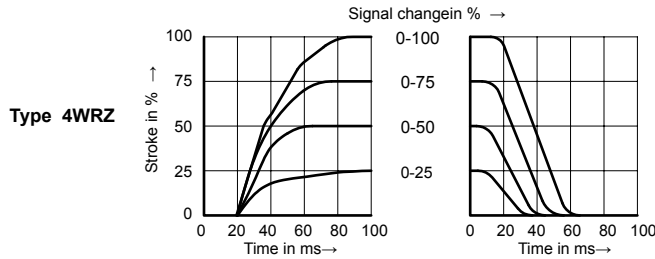
Transient function with a stepped form of electrical input signal P_{st} = 50\text{bar}
