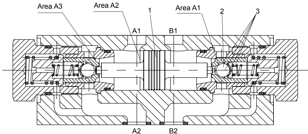
Z2S10..3XJ/...modular hydraulic check valve
